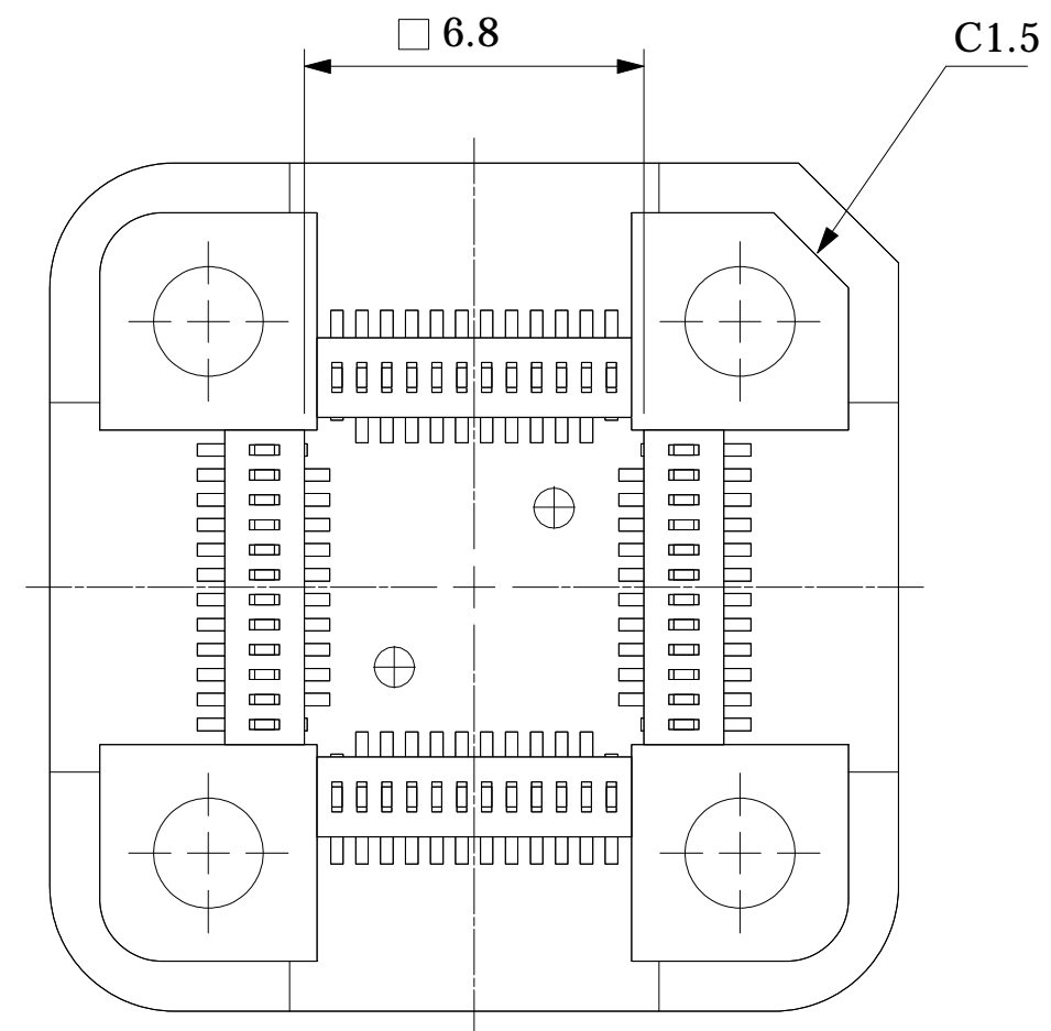
BOTTOM VIEW
