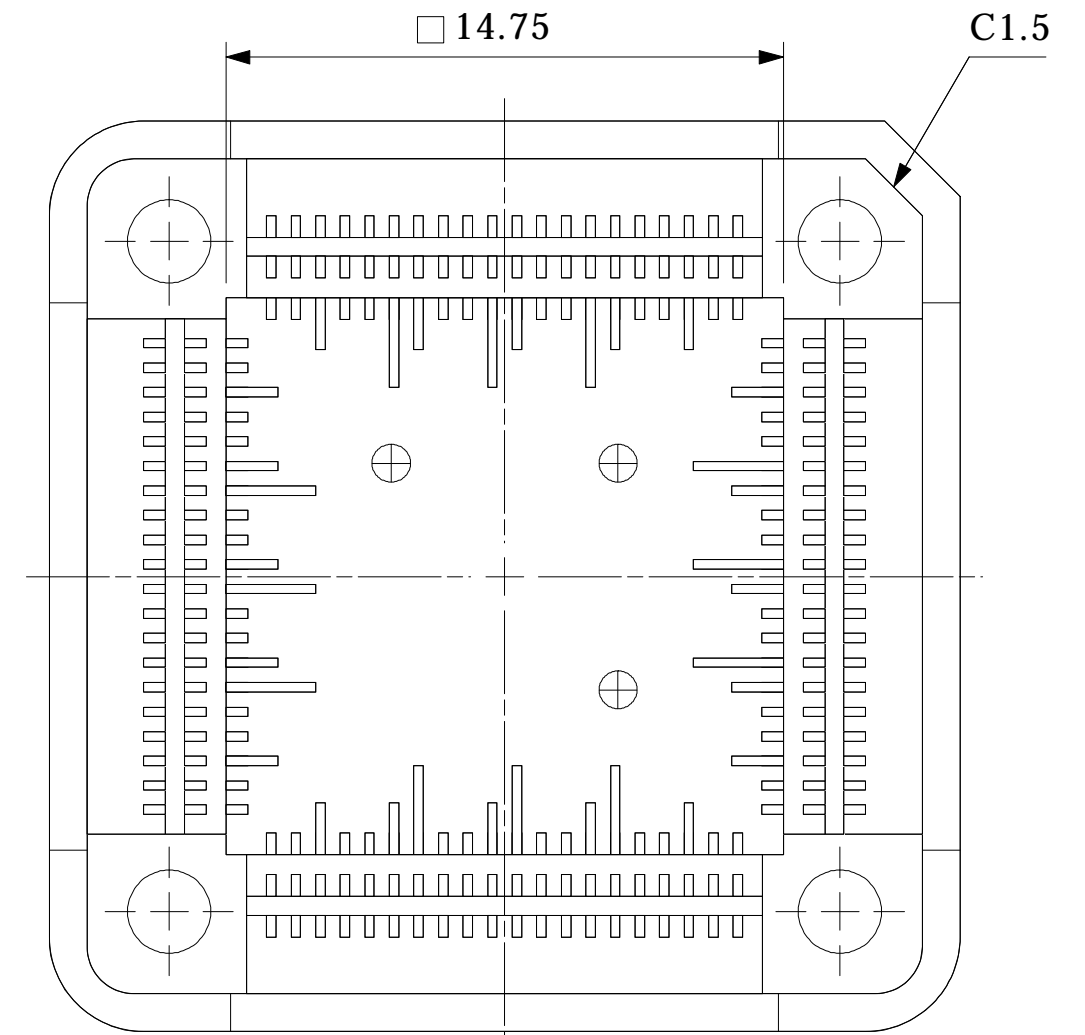
BOTTOM VIEW
